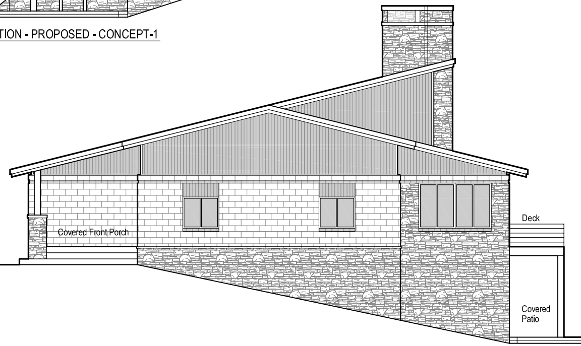
EAST ELEVATION - PROPOSED - CONCEPT-1
