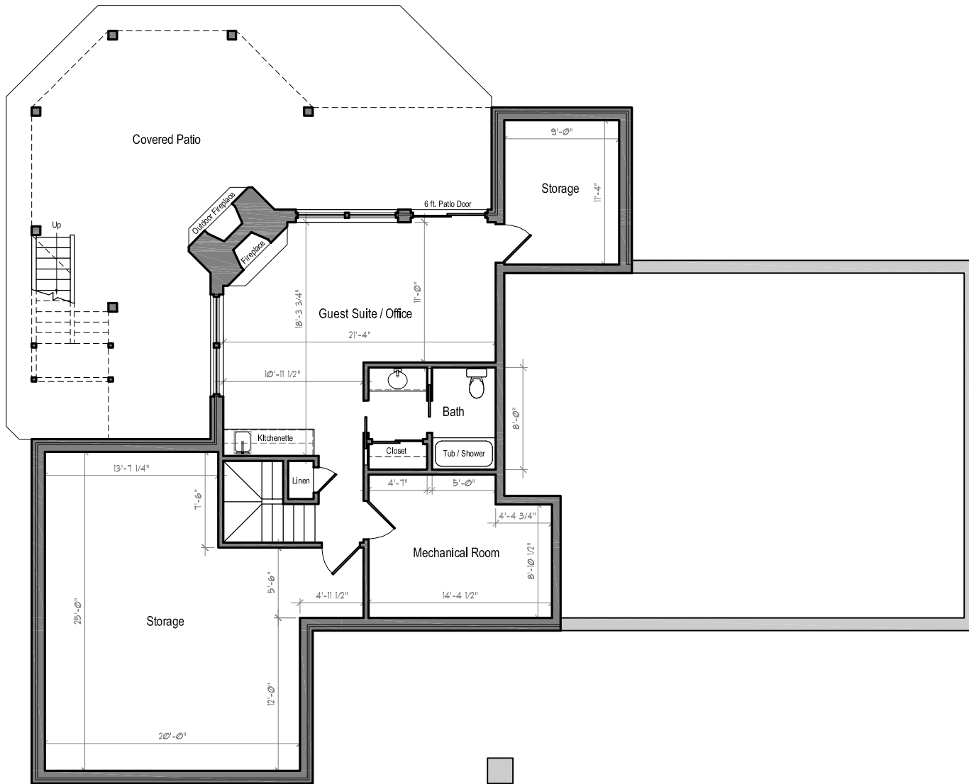
BASEMENT PLAN - PROPOSED - CONCEPT-1
