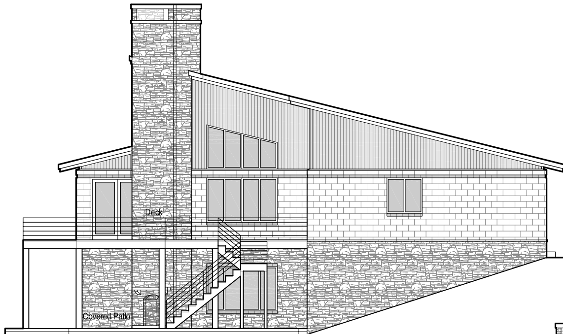
WEST ELEVATION - PROPOSED - CONCEPT-1
